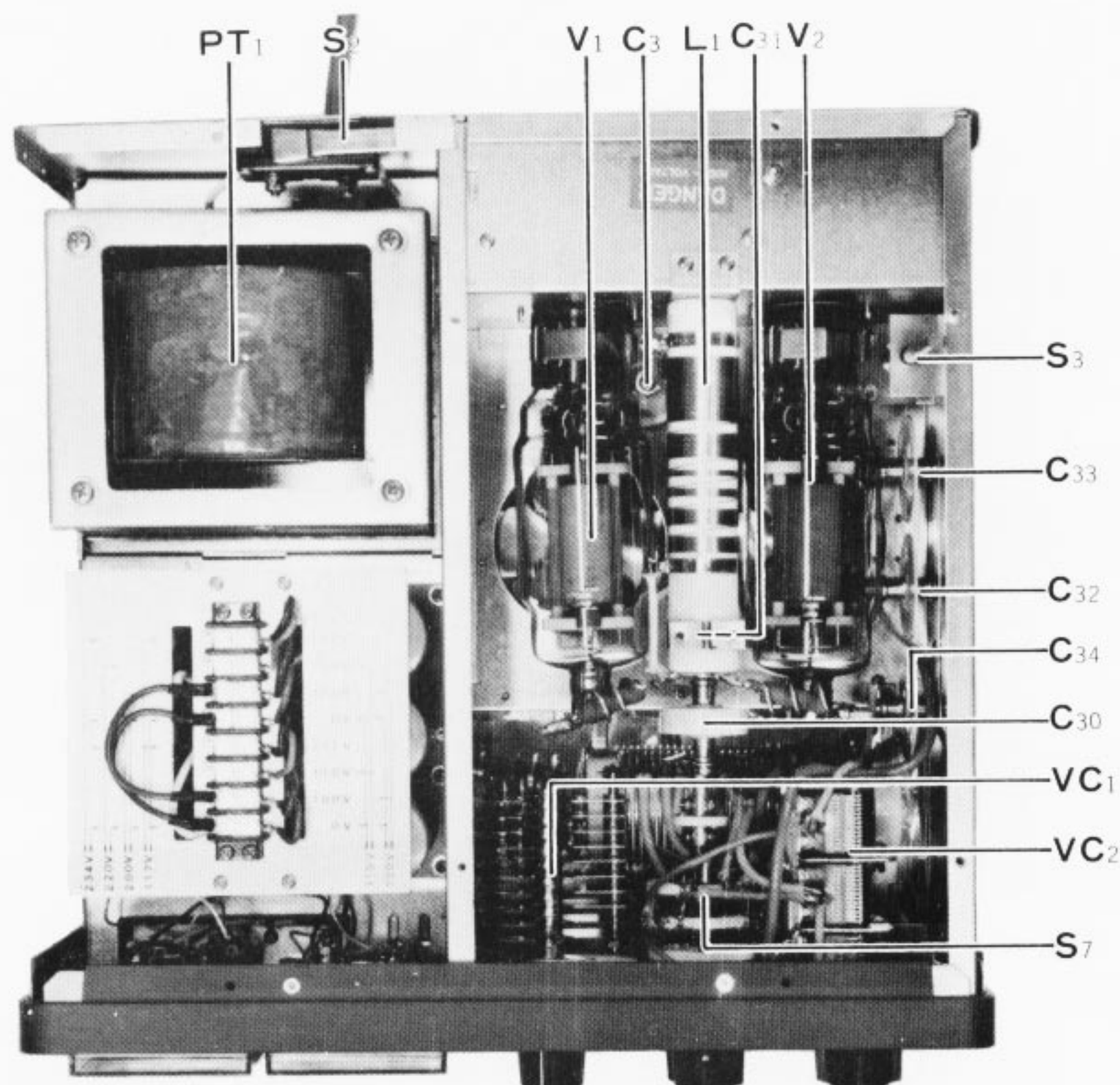
TOP VIEW
